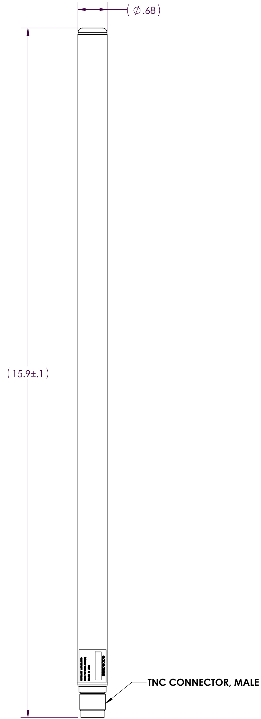
FRONT VIEW
